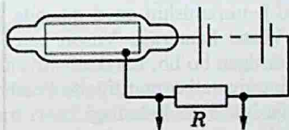
Geyger hisoblagichi
